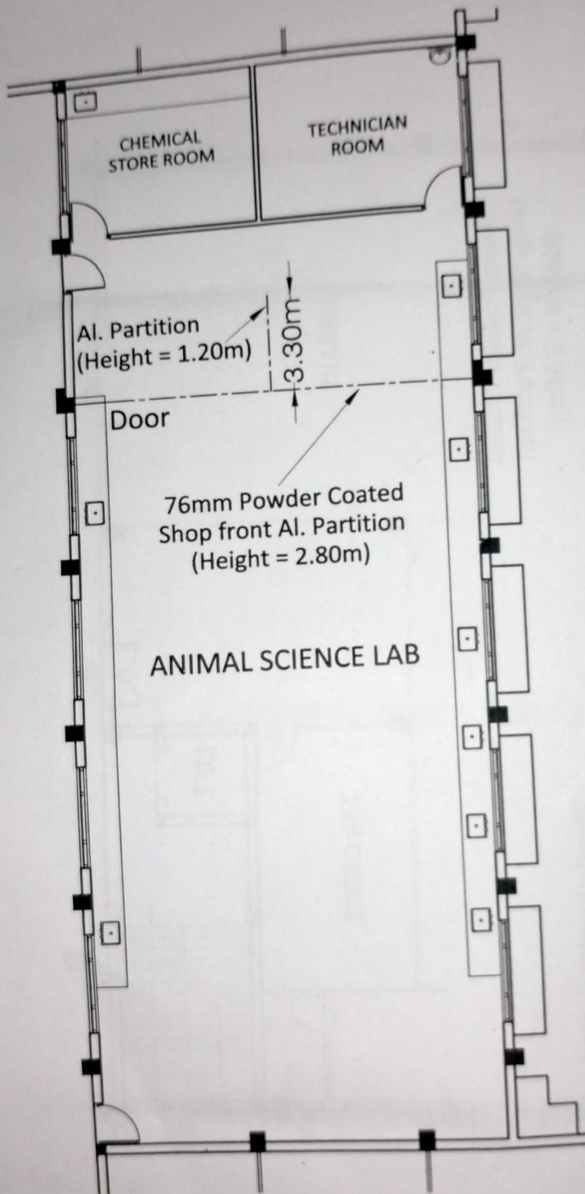
Partition Layout at Animal Science Faculty of Agriculture, Palachcholai, EUSL
